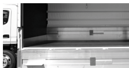
standard fittings: lateral pallet stop and smooth loading operation (inner front wall and corner posts on one level)
